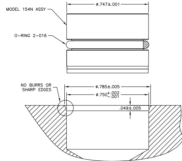
RECOMMENDED MOUNTING DIMENSIONS
