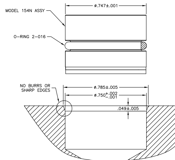
RECOMMENDED MOUNTING DIMENSIONS
