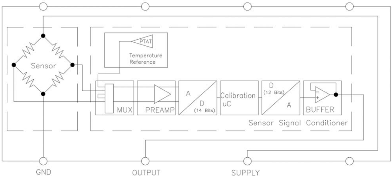
SAS55 Digital output
