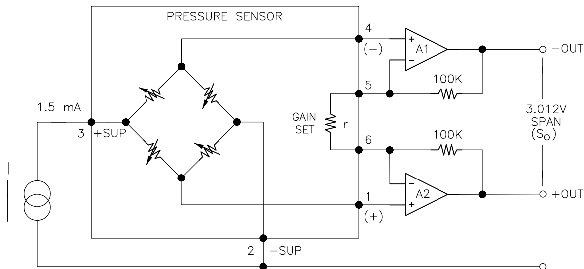
APPLICATION SCHEMATIC
