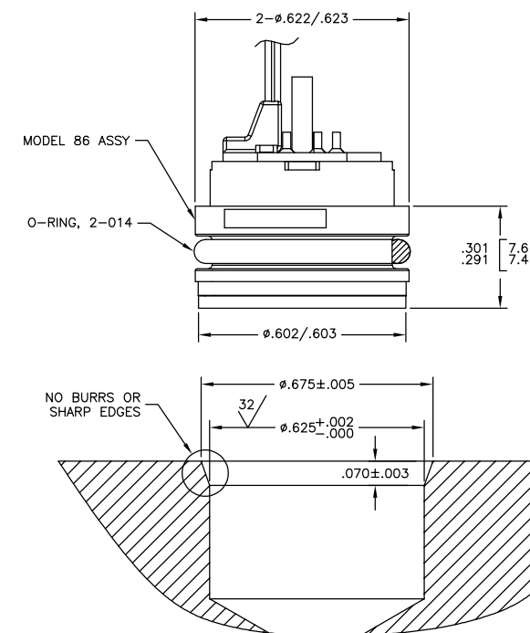
RECOMMENDED MOUNTING DIMENSIONS
